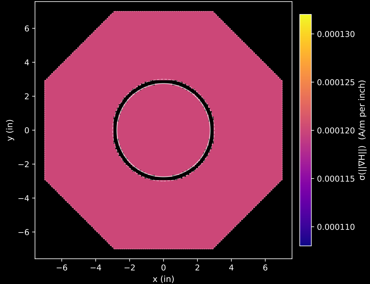
Propagated uncertainty
